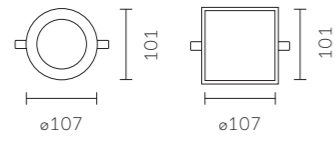
Arch Trimless
